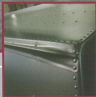
Full-length, oversized spray rails for a drier ride in rough water
